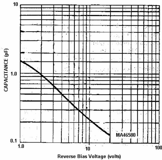
CAPACITANCE vs. VOLTAGE GAMMA = 1.25 +/-10% FROM 2-12V0lts
